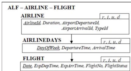
Figure 3. An example of \mathcal{F}_{Basic} form type
