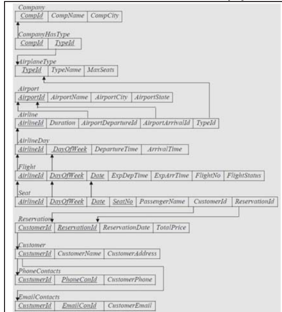
Figure 5. ATRS relational database schema
