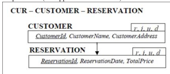
Figure 2. Form type Customer Reservations
