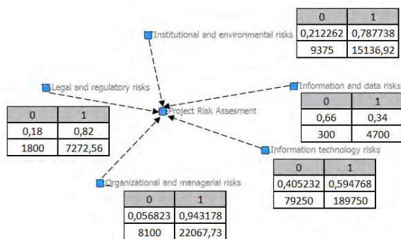
Figure 3. Integration of risk categories
