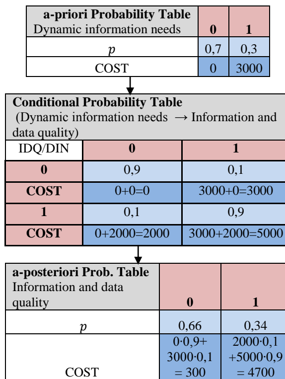
Figure 2. Example - calculation of a-posteriori probabilities and corresponding costs
