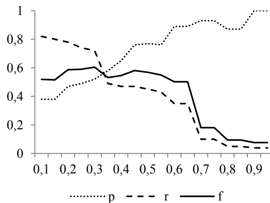
Figure 3. Evaluating N-Gram similarity
