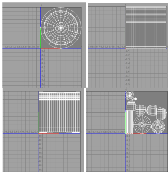
Figure 4. Test UV projection: planar, cylindrical, spherical, Automatic
